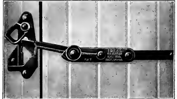
Automatic Freight Car Door Lock with Door About to Close
